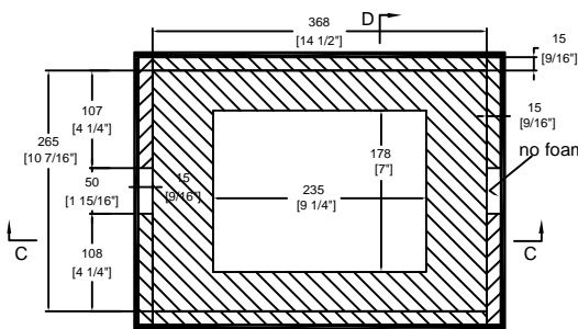
TOP VIEW OF BASE
