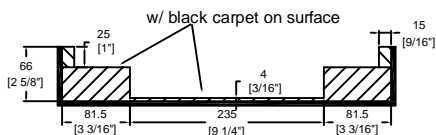
C-C VIEW
