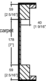
D-D VIEW
