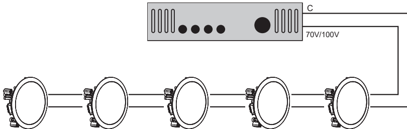
5 speakers connected in parallel using 20W Taps
