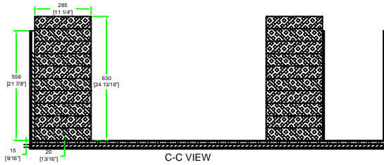
C-C VIEW
