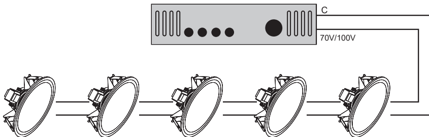
5 speakers connected in parallel using 6W Taps
