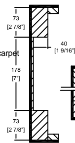
D-D VIEW
