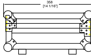
LEFT VIEW
