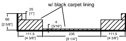
C-C VIEW
