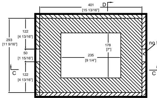
TOP VIEW OF BASE
