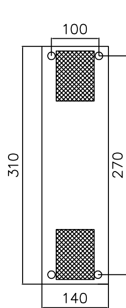
Top View
